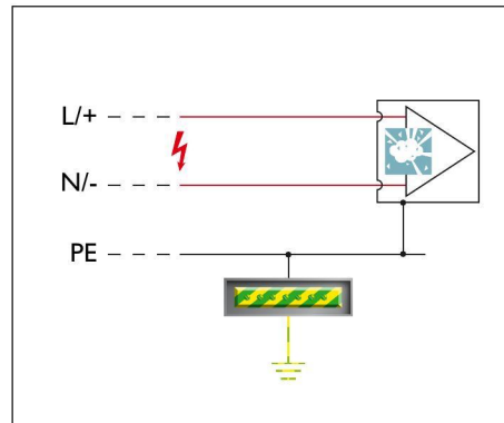
Fig. 8: Effects of a surge voltage as normal-mode voltage
