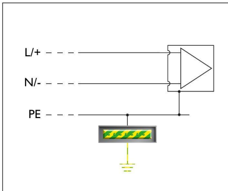
Fig. 7: Schematic power supply of a piece of equipment
